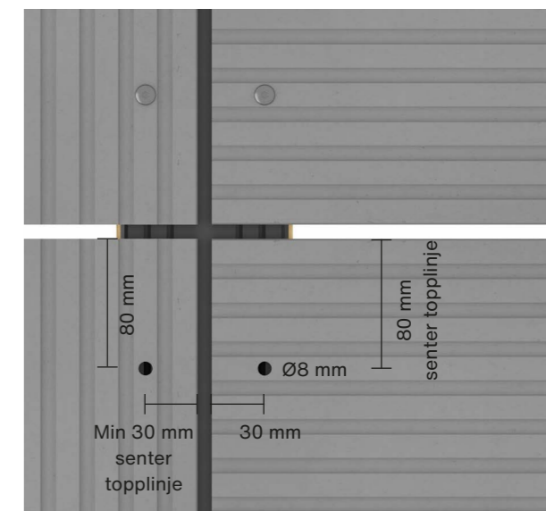
Fig 3. Swisspearl Patina Inline kantavstand
