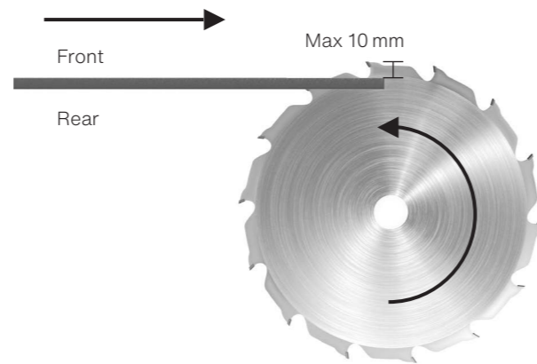
When using a table saw, place the board with the face up-most on the table and cut from the rear of the board.
