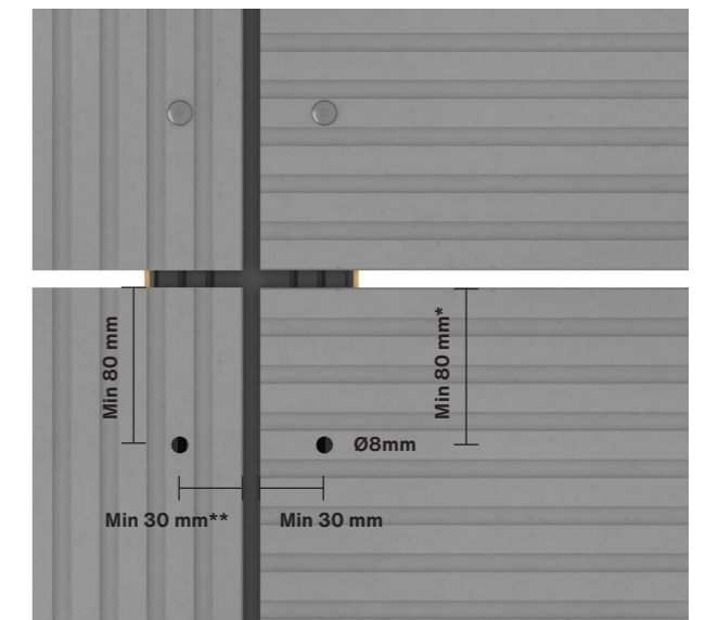
Fig. 3. Swisspearl Patina Inline Edge distances. Note! Min distance and/or the nearest following top line.
