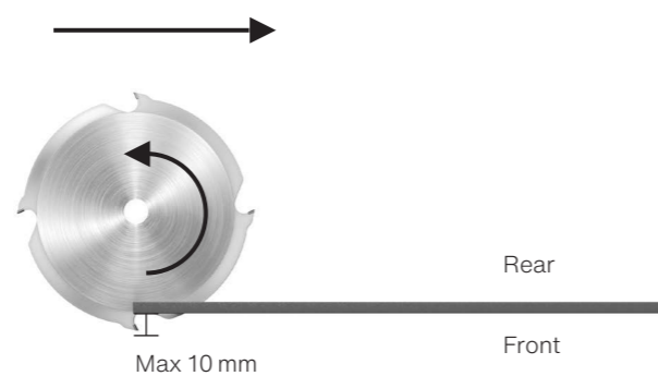
When using a circular saw or dive saw, cut the board from the rear.
