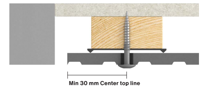
Fig. 4. Swisspearl Patina Inline installation of cut to size board.
