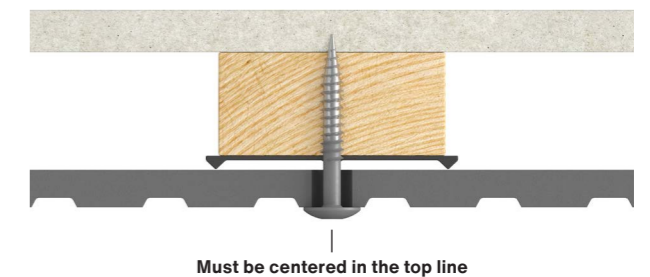
Fig. 2. Swisspearl Patina Inline installation on intermediate batten.
