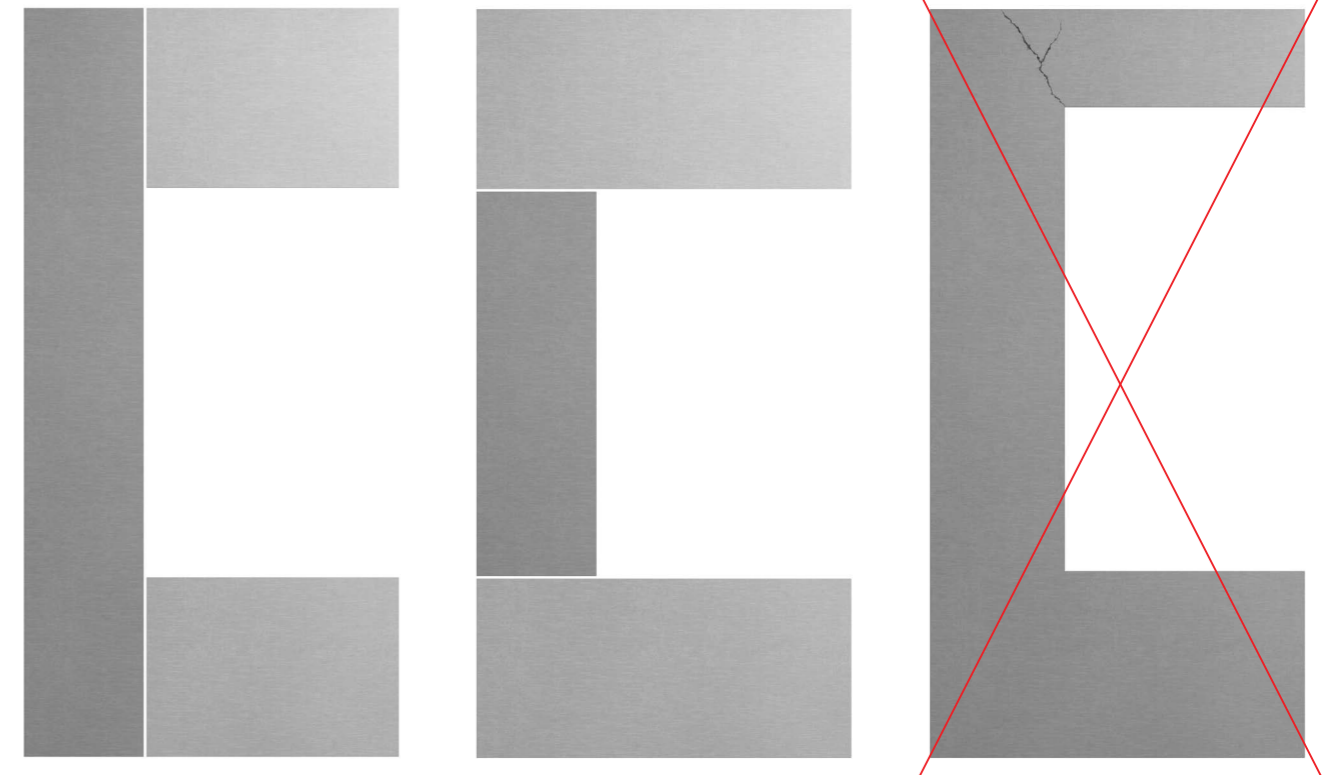
Correct installation of Swisspearl facade boards at windows, doors and openings.
