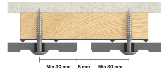
Fig. 1. Swisspearl Patina Inline installation on intermediate batten.
