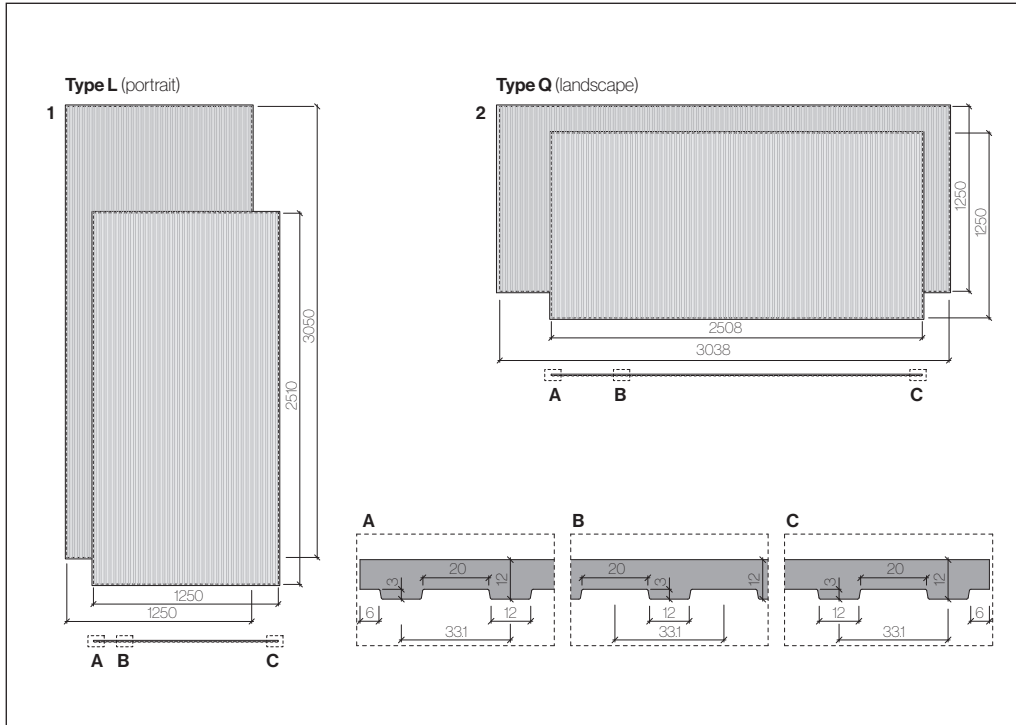
Graviat 9/12 mm thick panels - max. net panel sizes
