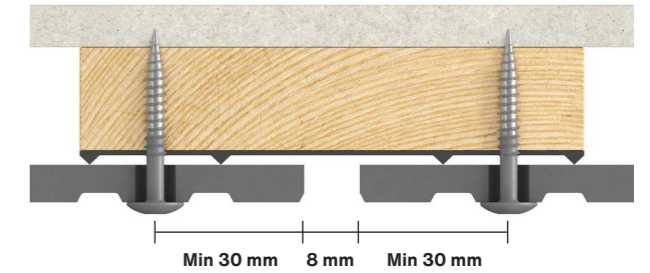
Fig. 1. Swisspearl Patina Inline installation on intermediate batten.
