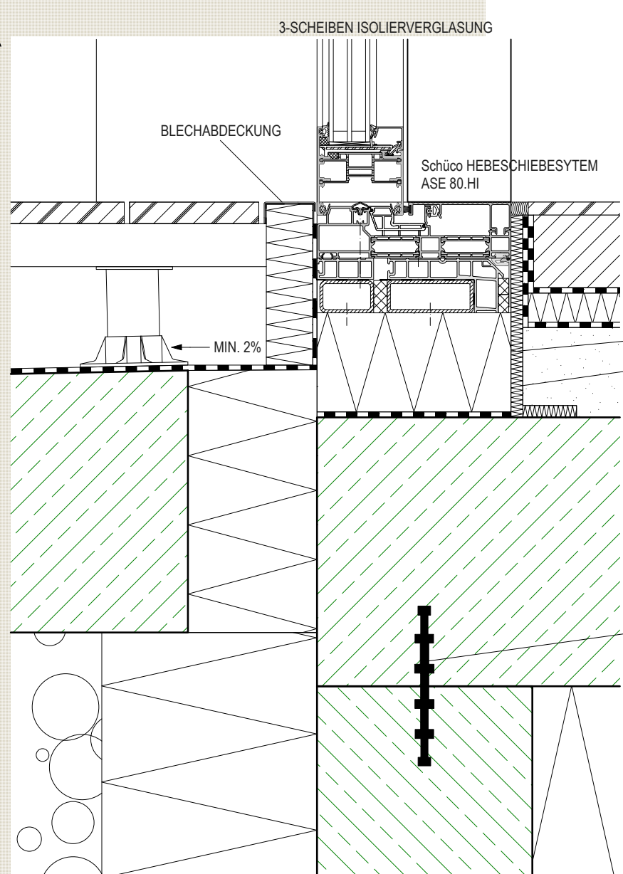
DETAIL A M 1:5
