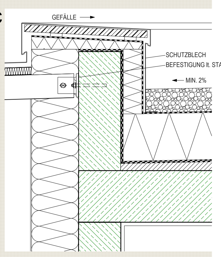
DETAIL C M 1:10
