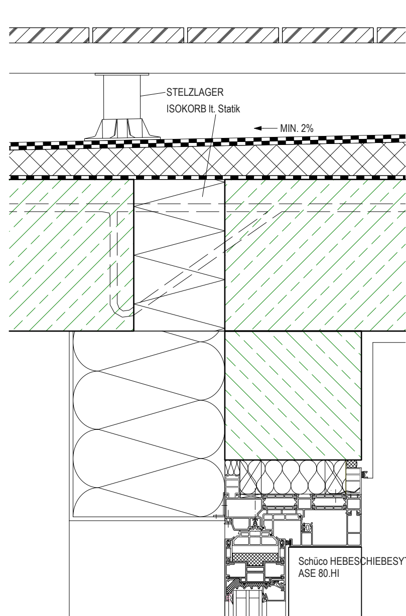
DETAIL B M 1:5
