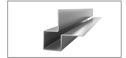
Swisspearl External Corner small Painted Aluminium Thickness 1.0mm Length 3000mm
