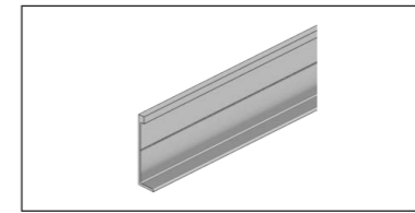
Swisspearl Plank Connect Vertical Start Profile Extruded Aluminium Thickness 1.1mm Length 3000mm
