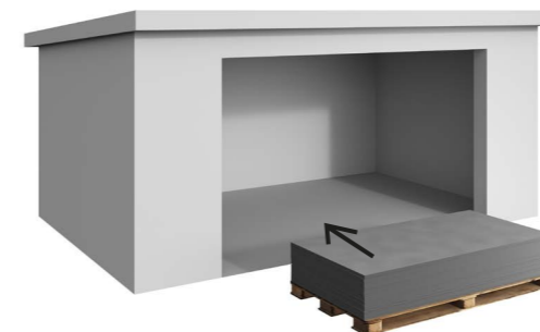
If Swisspearl facade boards are stored more than 2-3 weeks on site, the pallets should be kept under a roof to ensure dry and ventilated conditions.
