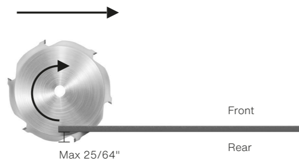
When using a mitre saw, cut the board from the front.
