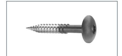
Swisspearl Facade Screw wood Without washer SCR-W 4.8x40 mm A4 stainless steel (Swisspearl Patina design line)
