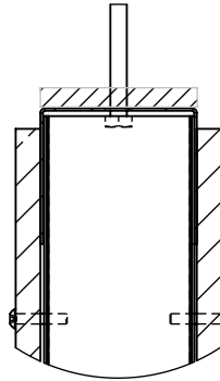
DETAIL C SCALE 1 : 4
